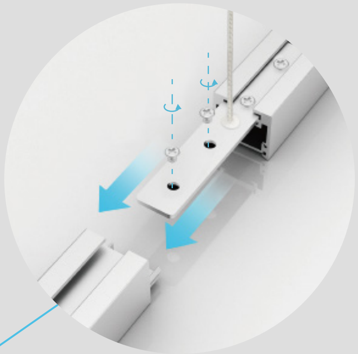
SVELT-D SVELT-CM SVELT-R Suspended Direct/Indirect (without end cap)
